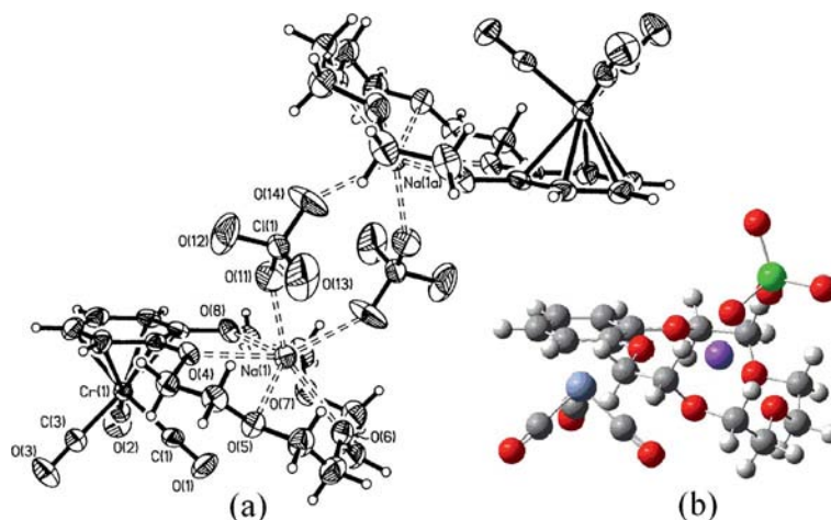
Figure 1. a: ORTEP drawing of the X-ray structure of [( 1 ·Na + ) ClO 4 − ] 2 ; b: corresponding view of the optimised structure (b3ylp/Lanl2DZ) from DFT calculations.
