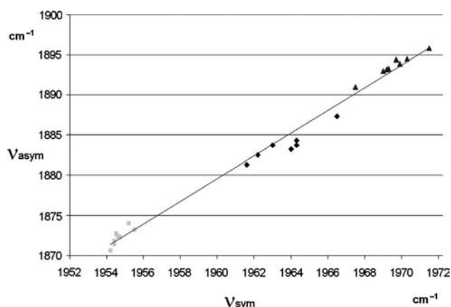
Figure 6. Bellamy plots of the frequencies of the symmetric and antisymmetric Cr–CO vibrational modes of 2 (squares), 1 (diamonds) and 3 (triangles); the trend line is from the data for all three complexes (the data point for 1 ·Ba 2+ was excluded).
