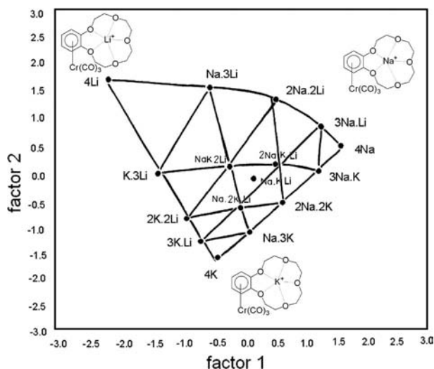
Figure 4. PCA factor score plot of spectroscopic data in the range 1890–1880 \text{cm}^{-1} from Figure 3.
