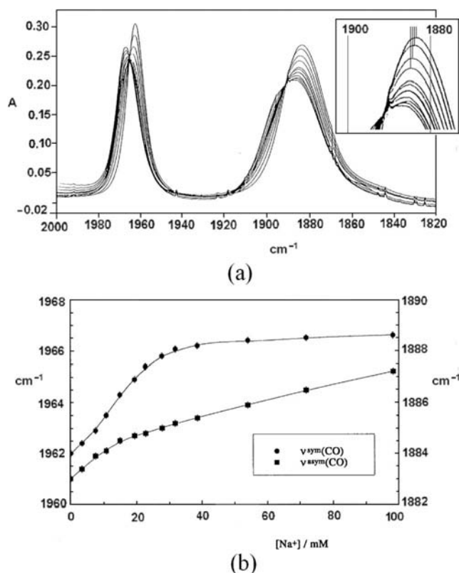
Figure 5. a: Superimposed FTIR spectra for 1 · \text{Na}^+ with [\text{Na}^+] varying from 0 to 98 mM [inset: expansion of the maxima observed for \nu_{\text{asym}}(\text{CO}) ]; b: positions of \nu_{\text{max}} for the \nu_{\text{sym}}(\text{CO}) and \nu_{\text{asym}}(\text{CO}) stretching vibrations plotted against [\text{Na}^+] .
