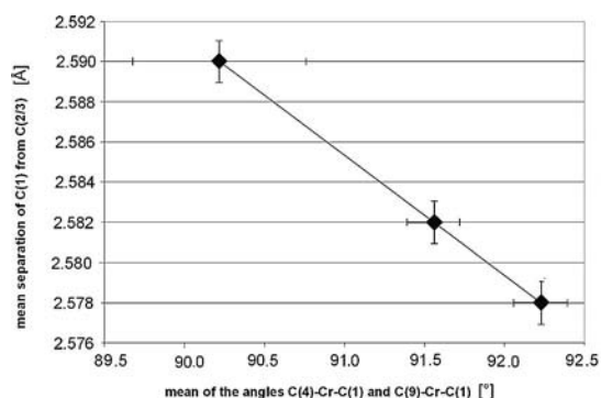
Figure 8. Plots of the means of the distances between \text{C}(1) and \text{C}(2) and between \text{C}(1) and \text{C}(3) (Table 3, line 21) against the mean of the angles \text{C}(4)–\text{Cr}–\text{C}(1) and \text{C}(9)–\text{Cr}–\text{C}(1) (Table 3, line 17).
