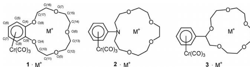
Figure 2. Metal cation adducts of tricarbylchromium derivatives 1 , 2 and 3 of crown ethers (atom labels on 1 correspond to numbering in the X-ray structure).
