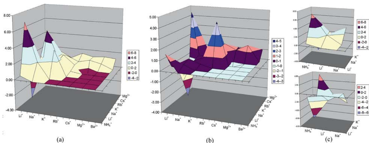
Figure 7. Plots of ratios of \Delta_{\text{N}} values (vertical axes) for pairs of \text{M}^+ ions [a: \Delta_{\text{N}(\text{1})}/\Delta_{\text{N}(\text{3})} ; b: \Delta_{\text{N}(\text{3})}/\Delta_{\text{N}(\text{1})} ; c: two views of \Delta_{\text{N}(\text{1})}/\Delta_{\text{N}(\text{3})} data from (a) to compare responses of 1 and 3 to \text{NH}_4^+ and the three alkali metal cations \text{Li}^+ , \text{Na}^+ and \text{K}^+ giving the PCA data in Figure 4].
