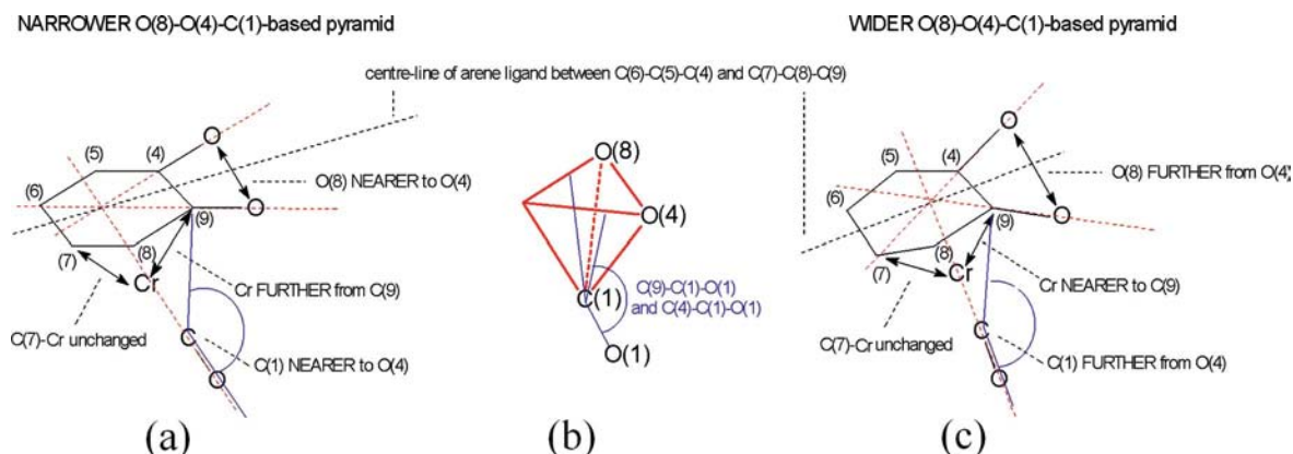
Figure 9. a: illustration of distortion of [O(4)-C(9)-C(4)-O(8)]Cr-C(1)=O(1) to form a narrower pyramid; b: the pyramid formed by extrapolating the bonds O(8)-C(4) , O(4)-C(9) and O(1)-C(1) towards the centre line between the C(6)-C(5)-C(4) and C(7)-C(8)-C(9) sections of the arene ligand, and the angles C(9)-C(1)-O(1) (at the front of the pyramid) and C(4)-C(1)-O(1) (at the back of the pyramid); c: illustration of distortion of [O(4)-C(9)-C(4)-O(8)]Cr-C(1)=O(1) to form a wider pyramid.
